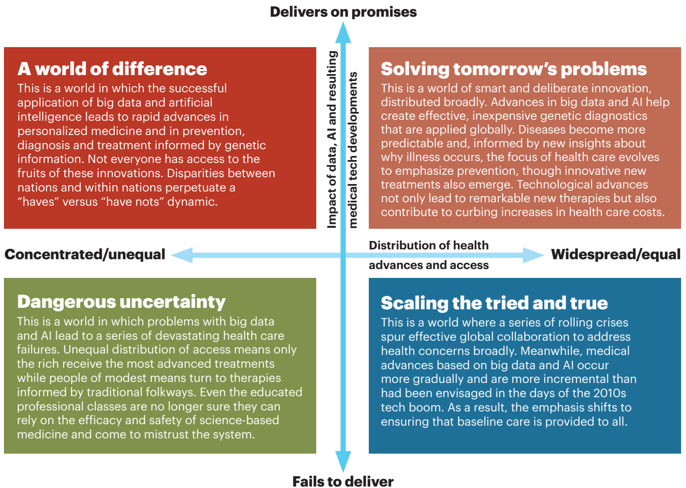
Figure 2: Scenarios developed in the Trust CoLab exercise
